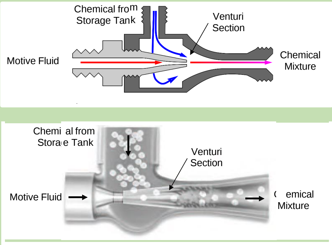
Figure 16: Section views of eductor jet pumps (nozzles).
