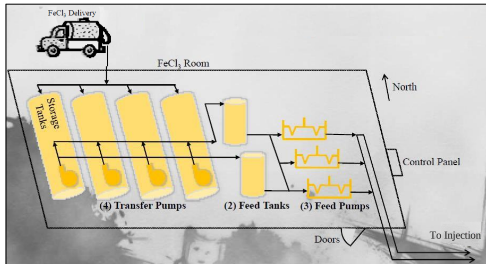
Figure 1: Schematic of a ferric chloride (FeCl 3 ) chemical feed system.
