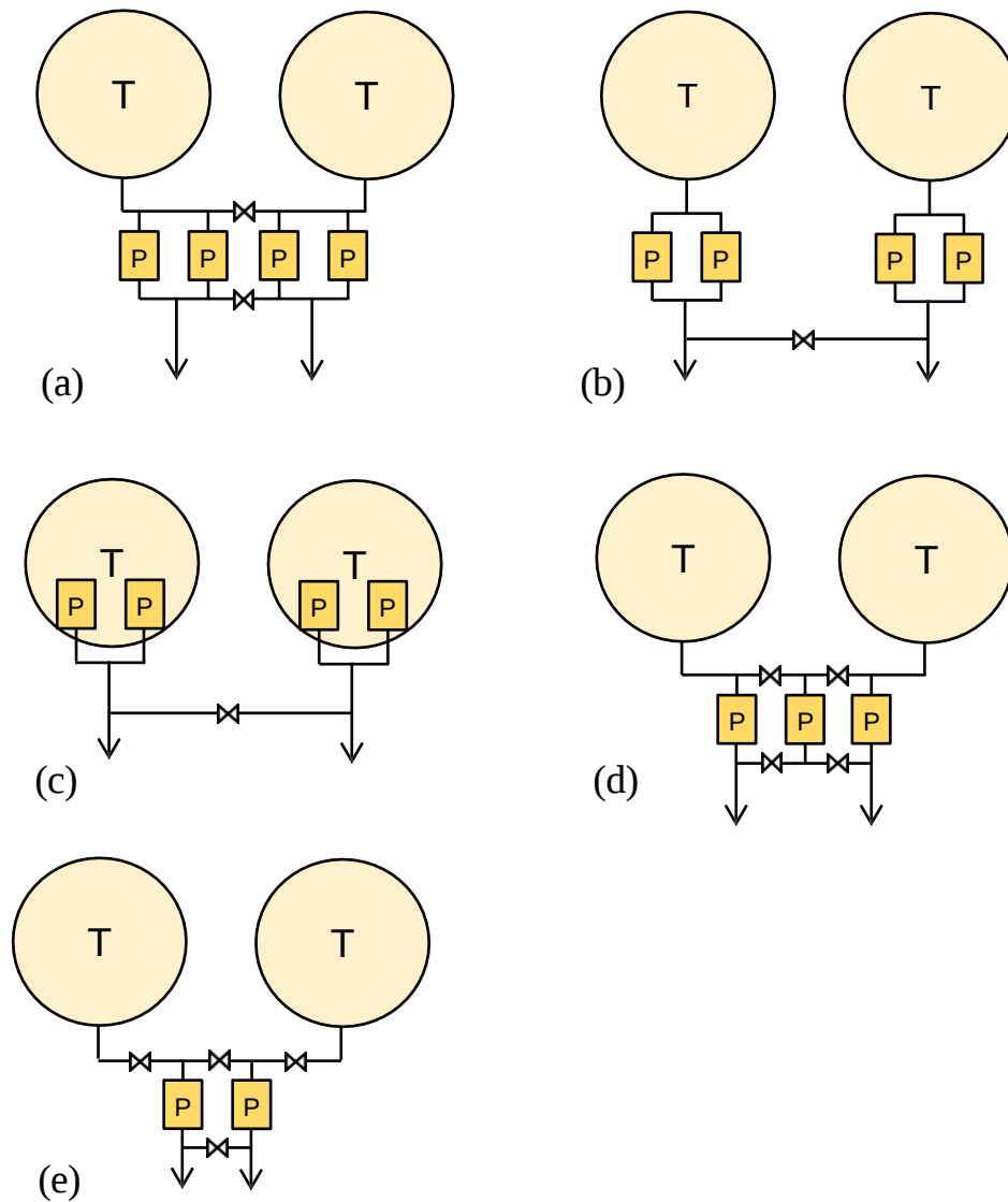
Figure 5: Alternative tank (T) and pump (P) arrangements to provide for redundancy of tanks, pumps, and piping. For (c), the pumps are mounted on top of the tanks.
