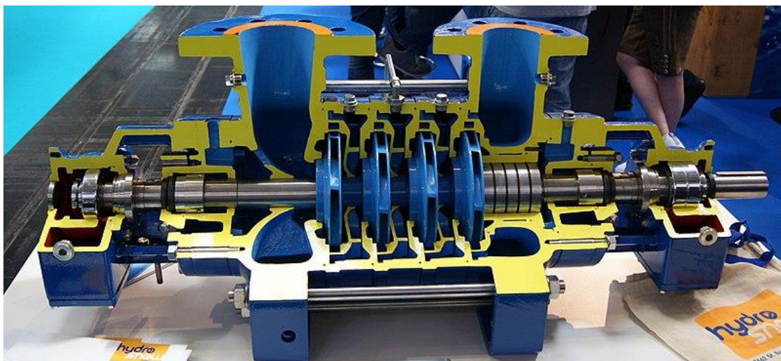
Figure 5: A multi-stage centrifugal pump with four impellers. Flow enters on the upper left and discharges on the upper right.
