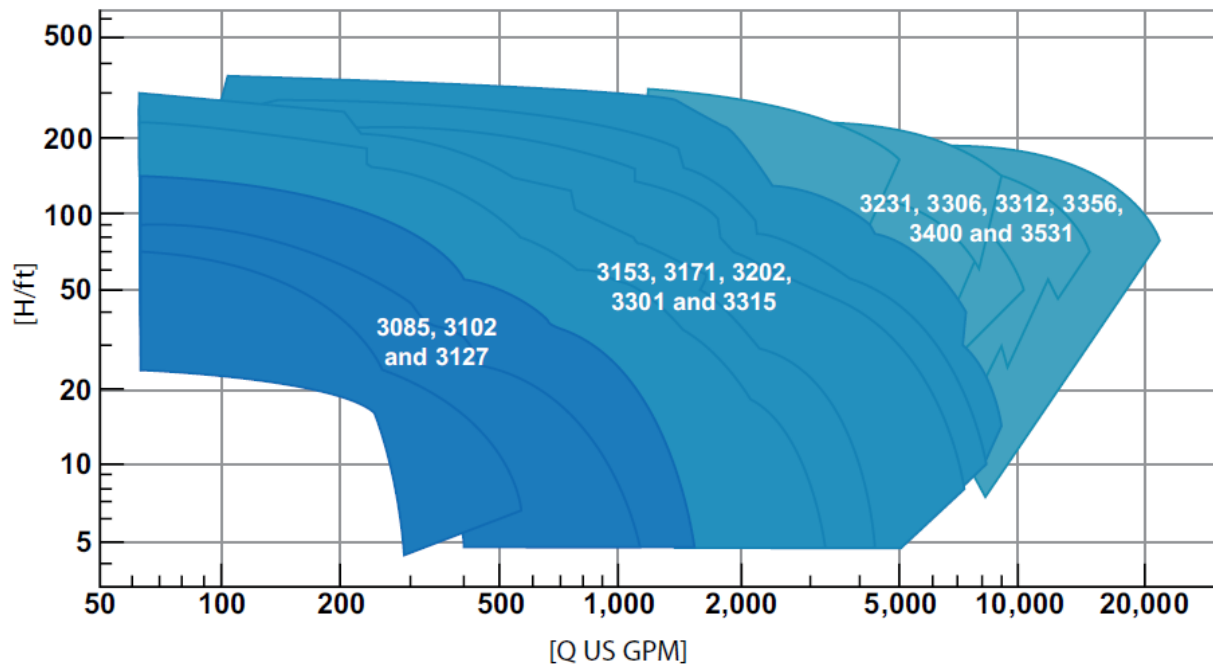
Figure 21: Example chart of capacity ranges for various pump model numbers.
