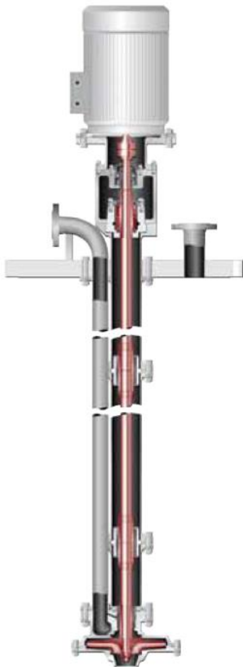
Figure 6: A vertical suspended column centrifugal pump for chemical pumping. The motor is mounted safely above the tank. The impeller is submerged near the bottom of the tank. A small discharge pipe rises to the left of the enclosed vertical shaft.
