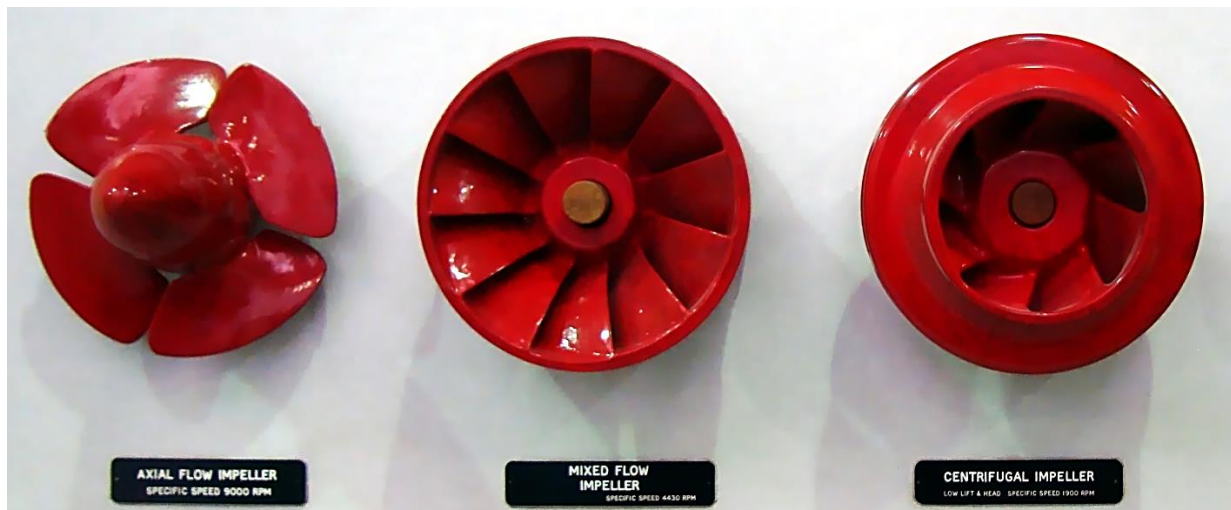
Figure 1: Example impellers for the three types of rotodynamic pumps.
