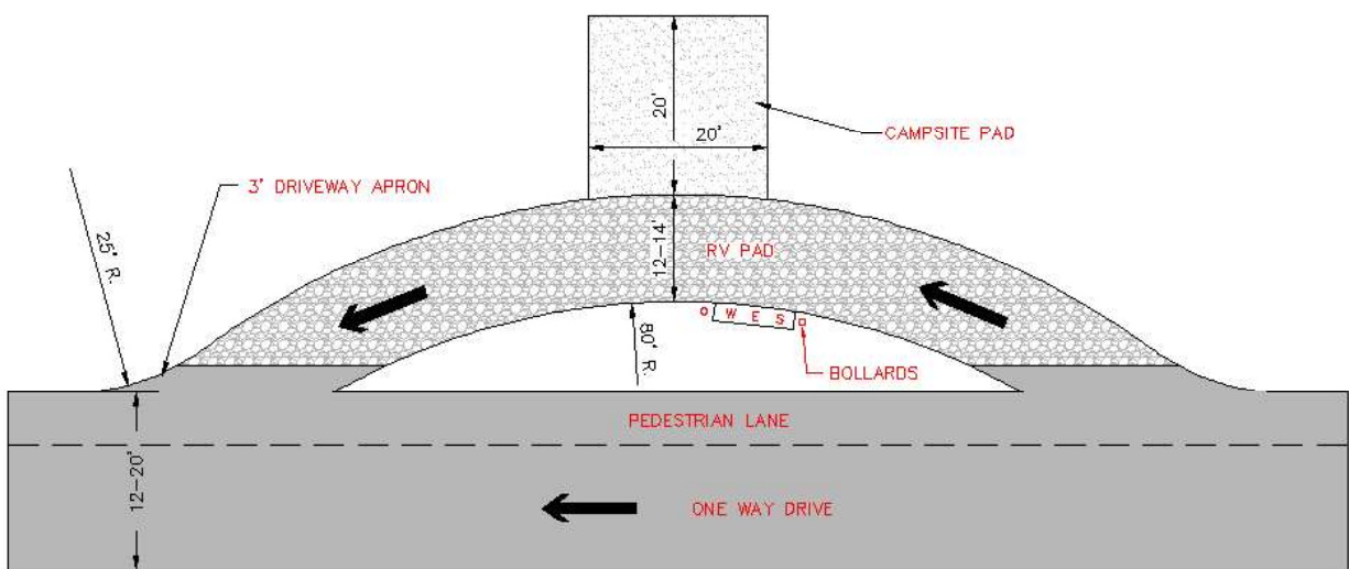
OUTSIDE LOOP PULL-THRU
