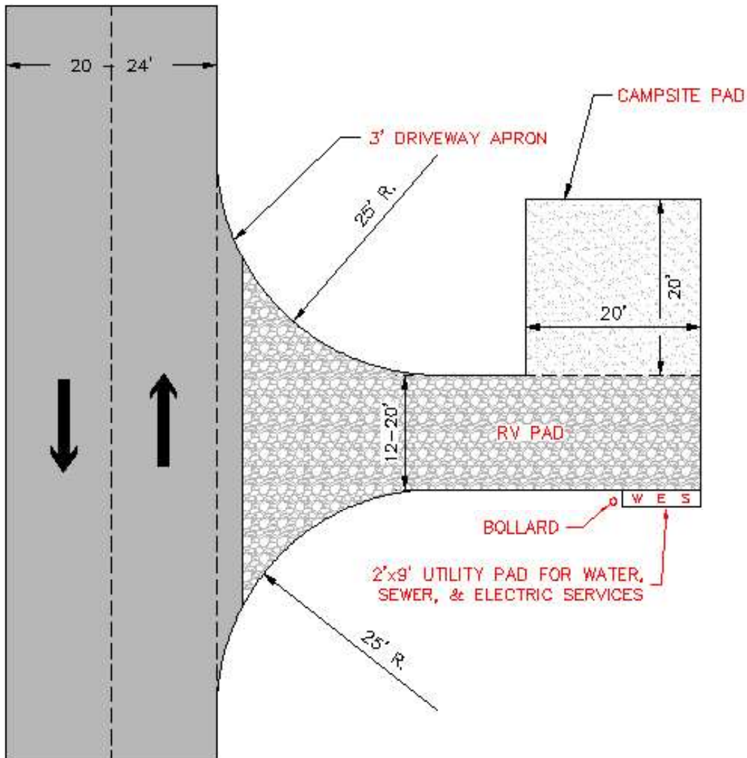
TWO-WAY DRIVE STRAIGHT BACK-IN
