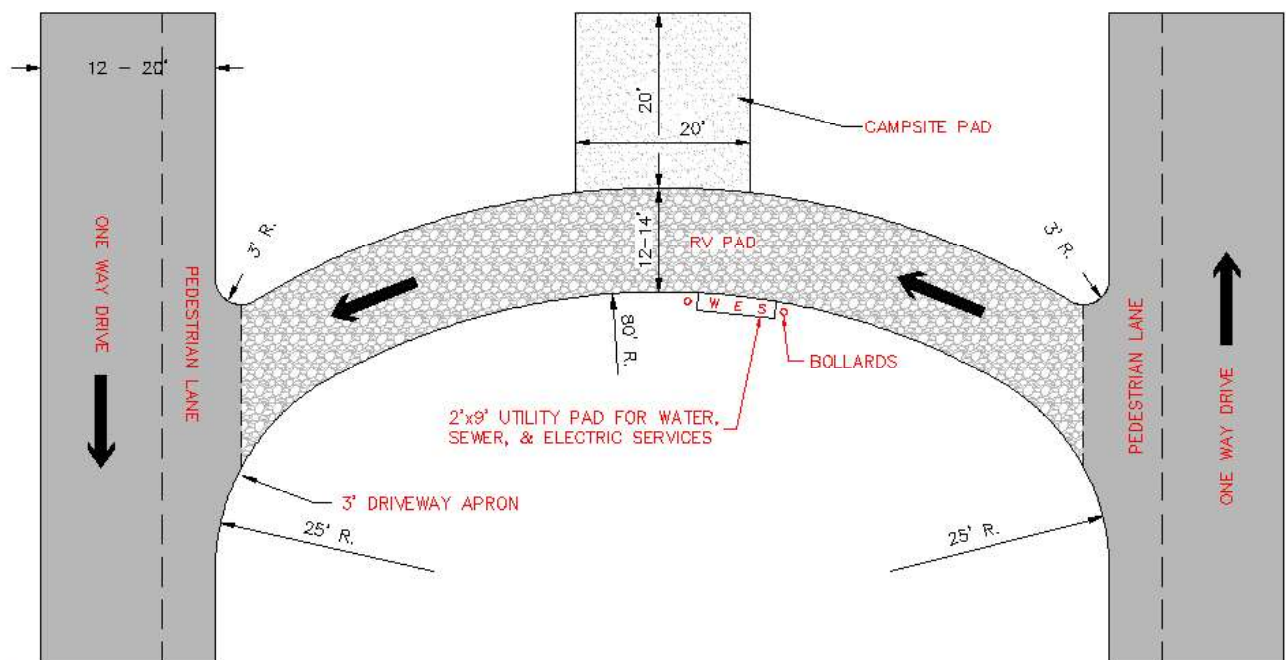
INSIDE ONE-WAY LOOP PULL THRU
