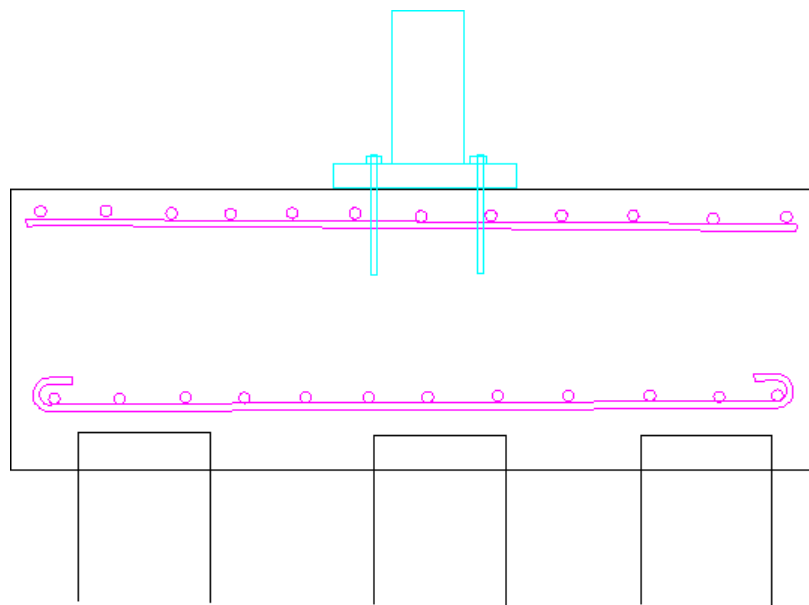
Typical Reinforced Concrete Pile Cap
