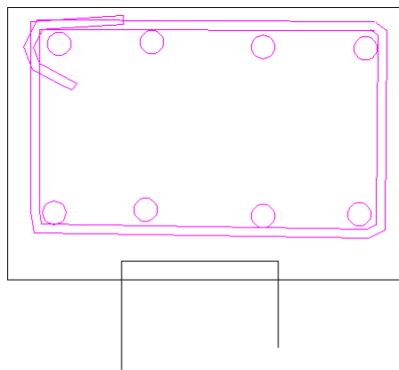
Grade Beam on Pile
