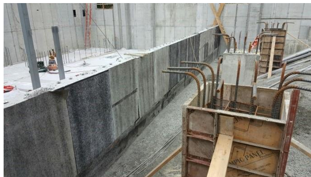
Piers for future columns above. And with steel column embedded (left)
