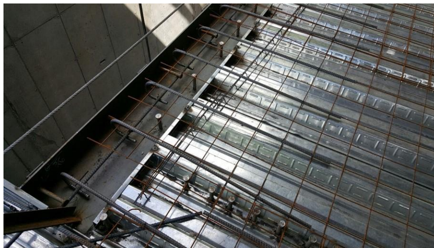
Slab on metal deck with wire and candy cane 180 hooks
