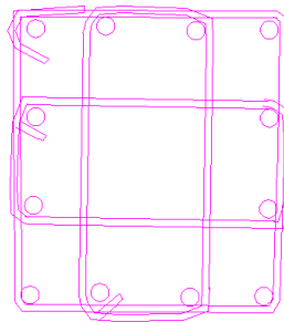
Pier Cross Section Plan With Inside and Outside Ties
