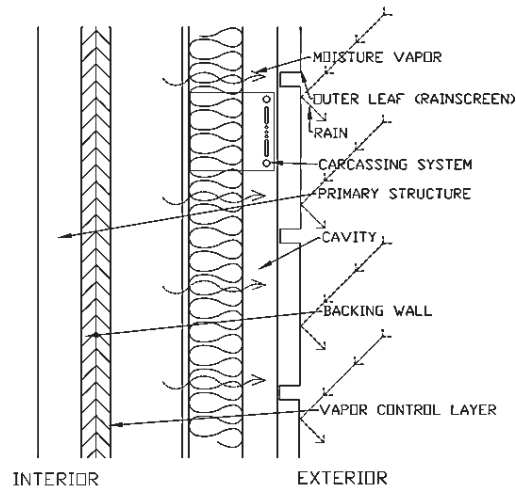
Diagram of a rain screen
