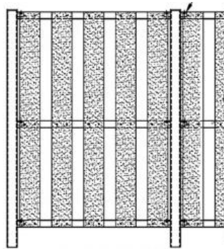
Aluminum Slat Divider
