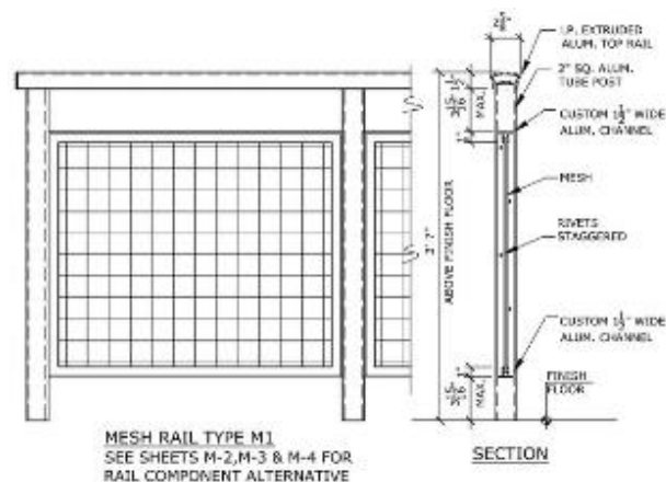
Mesh Rail Schematic
