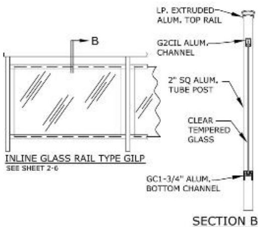
Glass Rail Schematic
