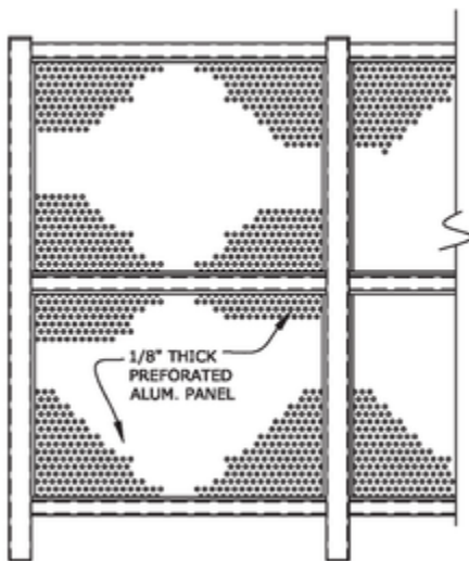
Perforated Mesh Divider
