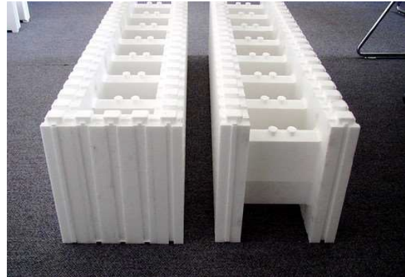
Insulating Concrete Forms
