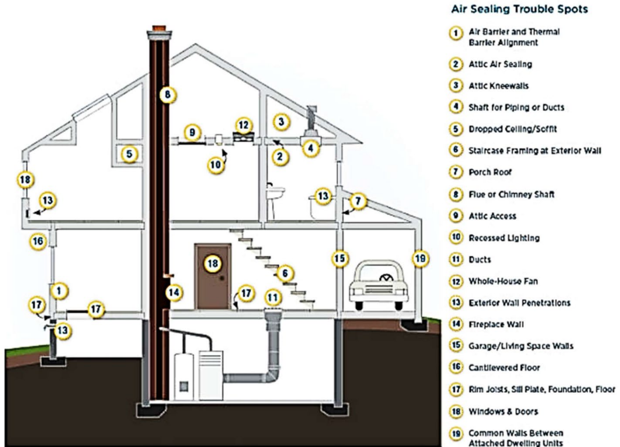
Common Trouble Spots—USDOE
