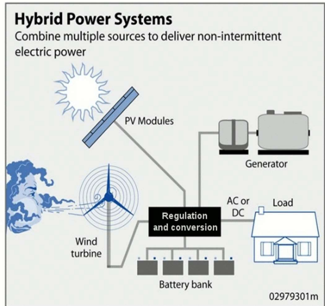
Hybrid Wind and Solar
