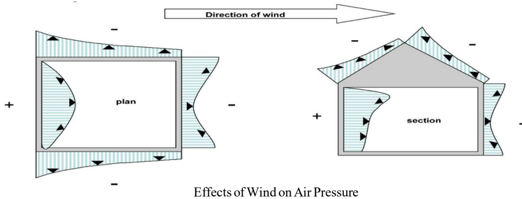
Effects of Wind on Air Pressure
