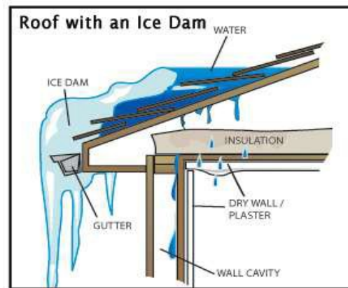
Badly Vented Roof
