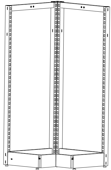
MAXe INSIDE CORNER SECTION WITH CORNER SKIRT SET
