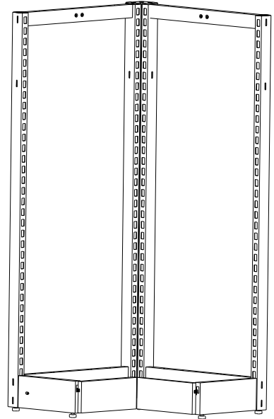
MAXe INSIDE CORNER SECTION WITH CORNER SKIRT SET
