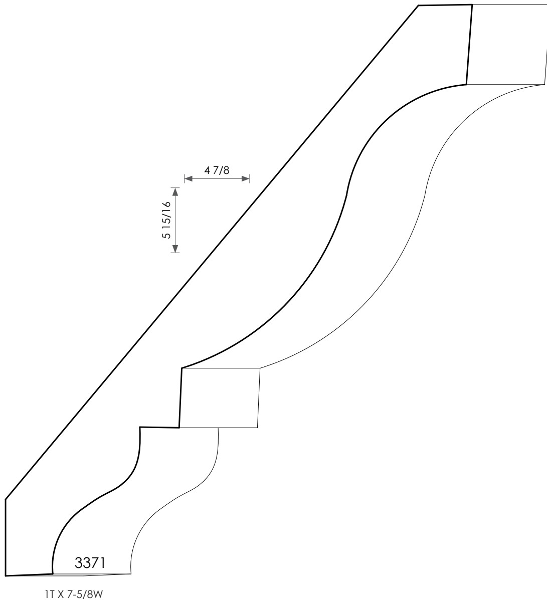
Wood Crown Mold - 3371
