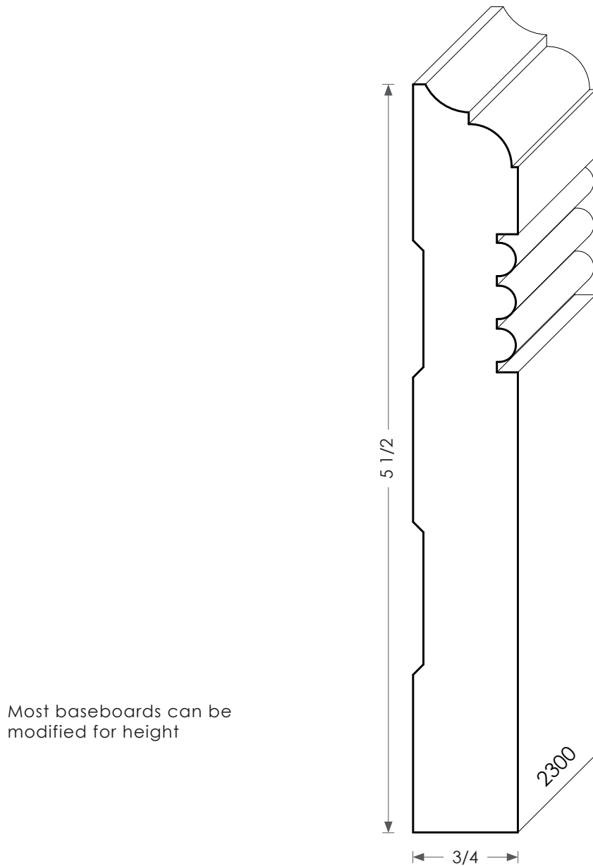
Wood Baseboard - 2300
