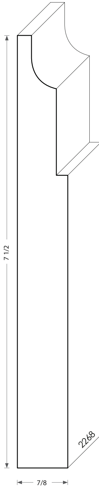
Wood Baseboard - 2268
