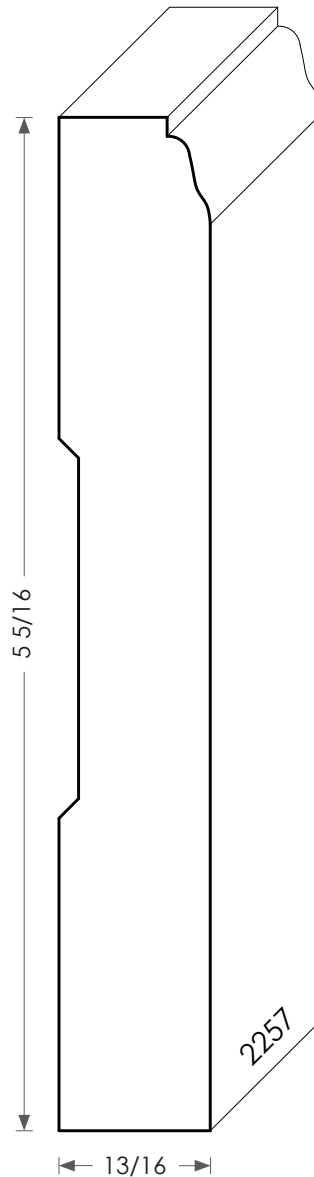
Wood Baseboard - 2257
