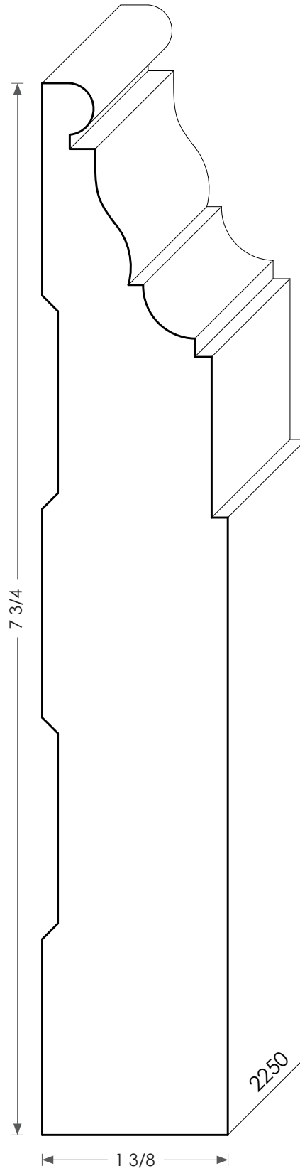
Wood Baseboard - 2250
