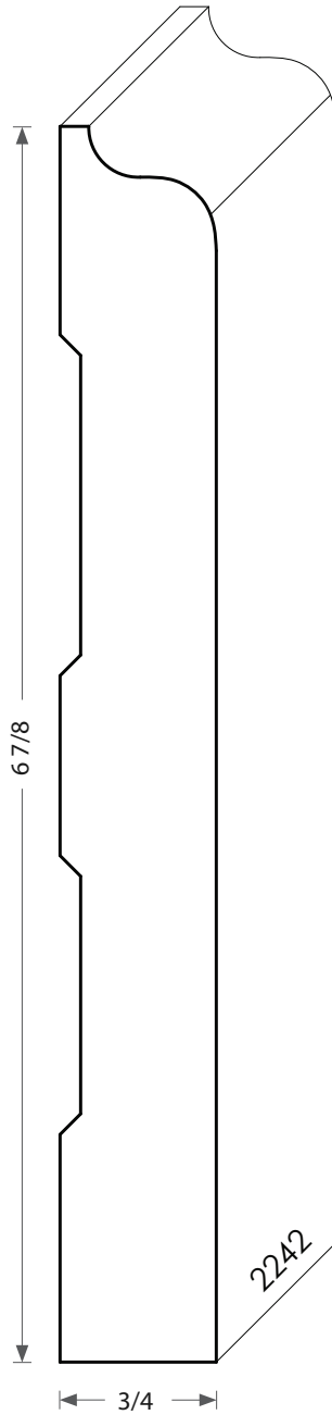
Wood Baseboard - 2242
