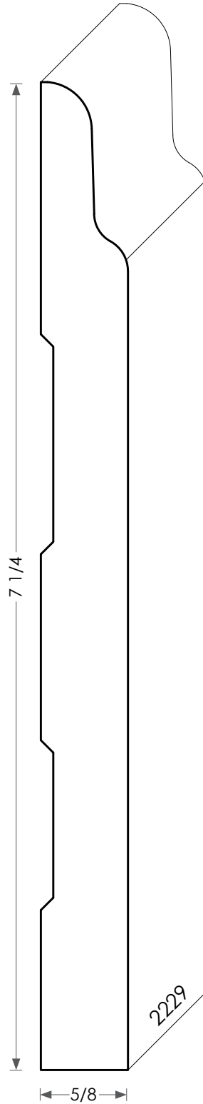
Wood Baseboard - 2229
