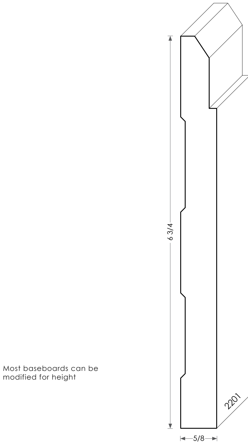
Wood Baseboard - 2201
