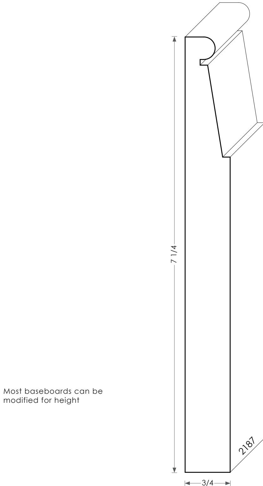
Wood Baseboard - 2187
