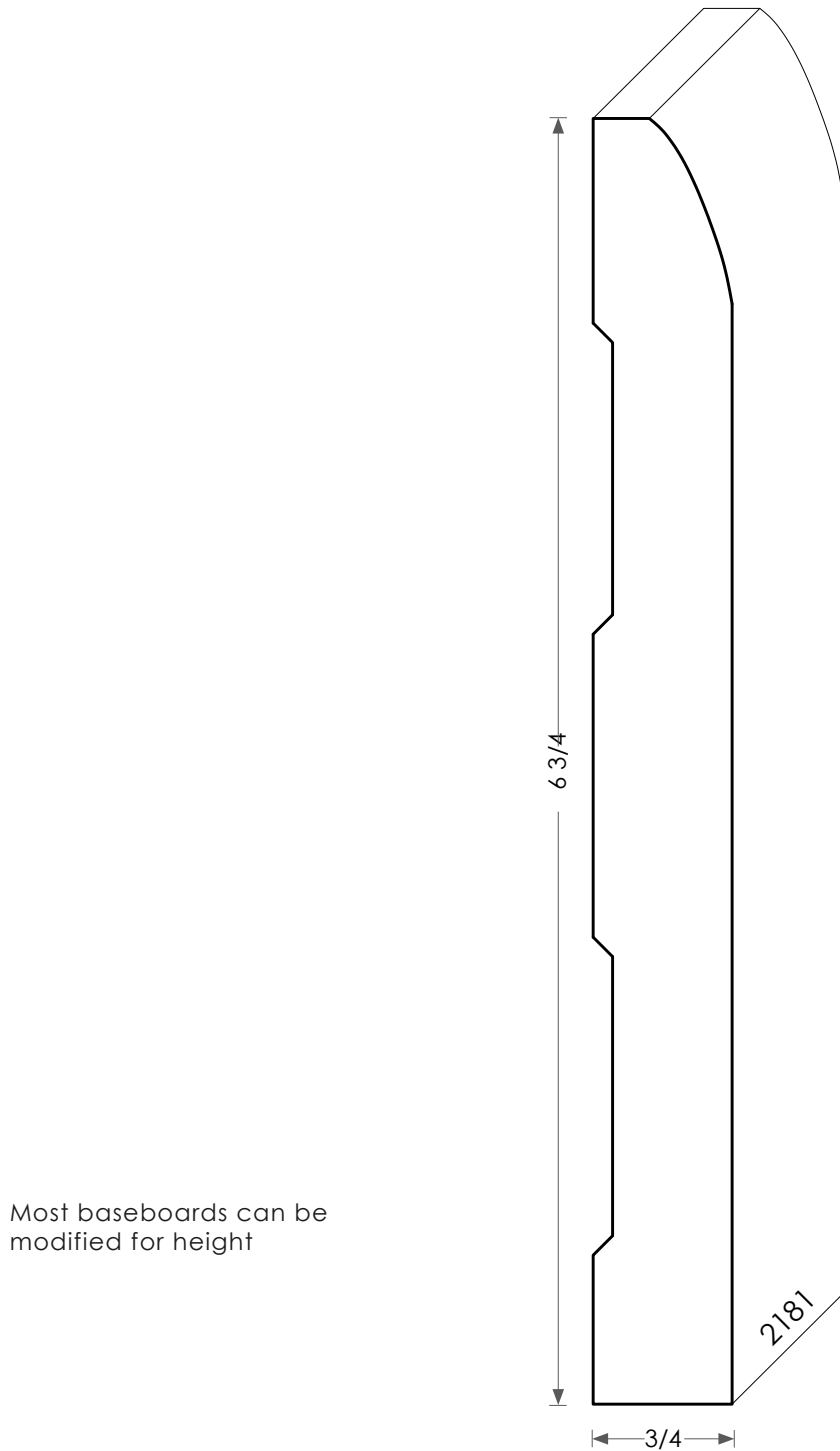
Wood Baseboard - 2181
