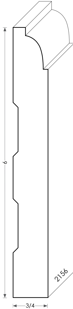
Wood Baseboard - 2156
