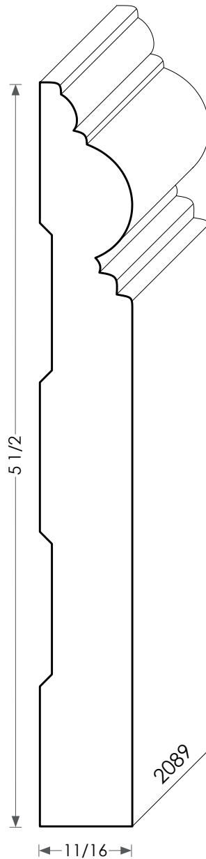
Wood Baseboard - 2089
