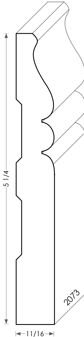
Wood Baseboard - 2073
