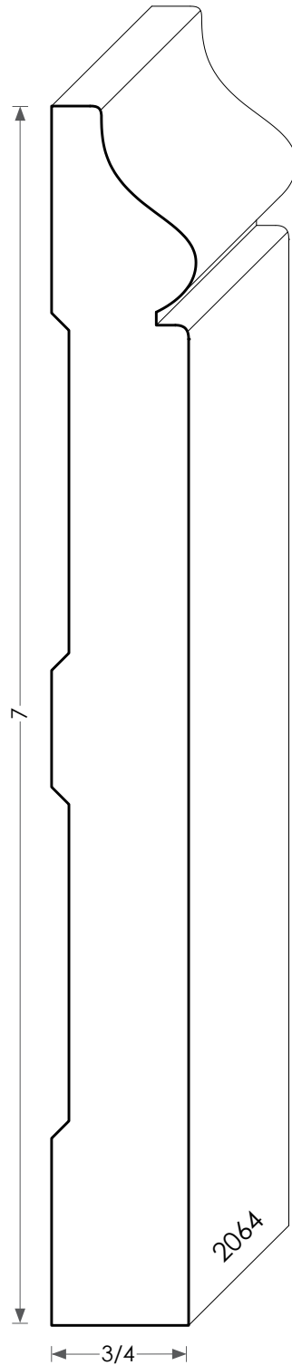
Wood Baseboard - 2064
