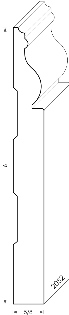
Wood Baseboard - 2052
