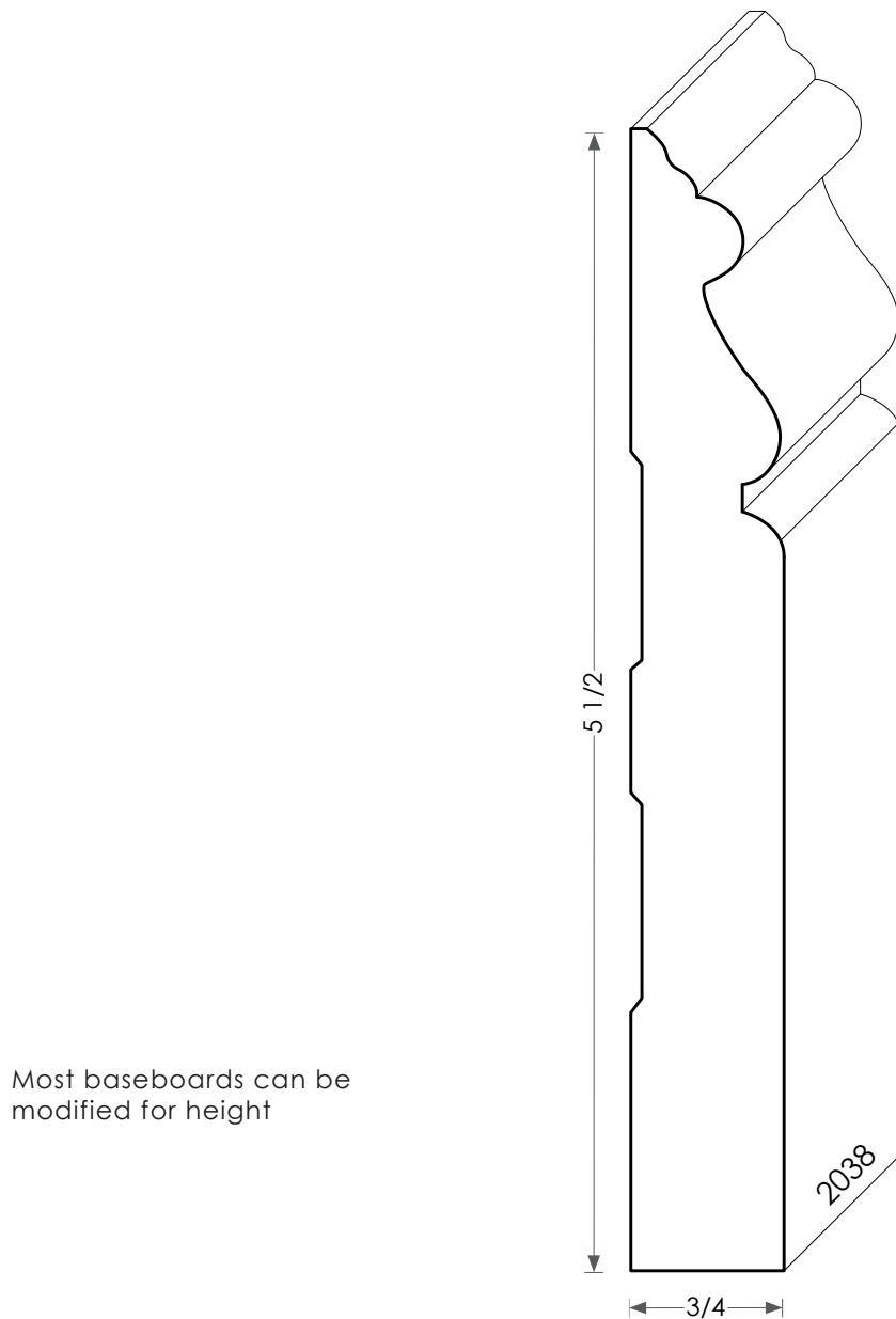
Wood Baseboard - 2038
