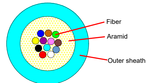
Cable Structure
