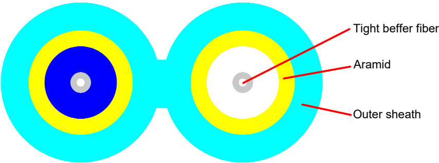
Cable Structure
