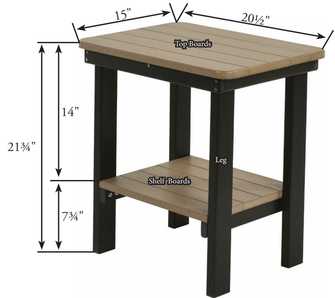
Rectangular End Table
