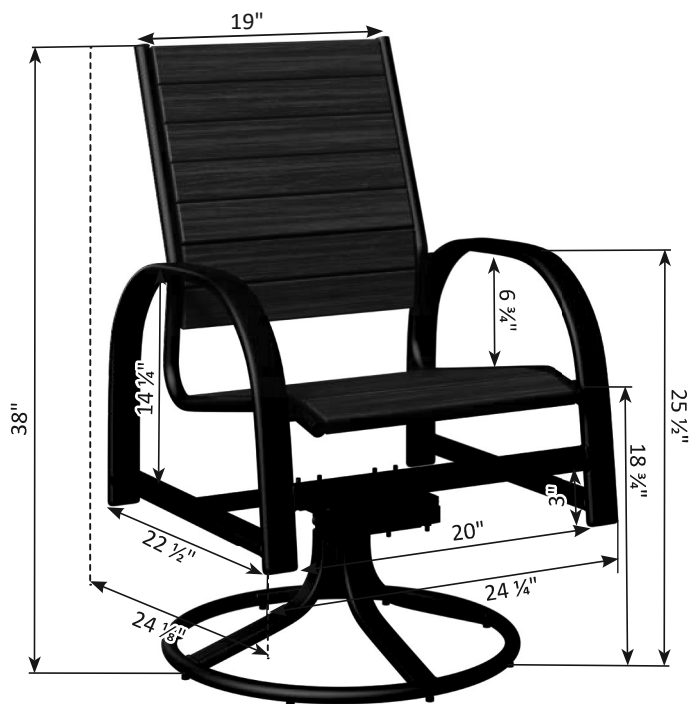
Murphy Dining Height Poly Swivel Rocker
