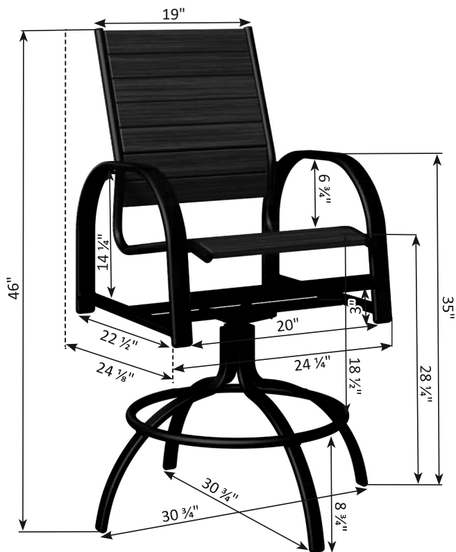
Murphy Bar Height Poly Swivel Chair
