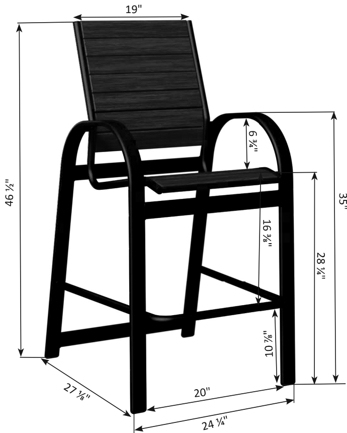
Murphy Bar Height Poly Chair
