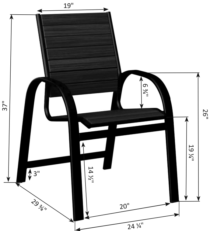
Murphy Dining Height Poly Chair
