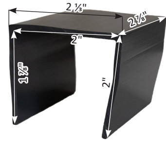
Sectional Connector
