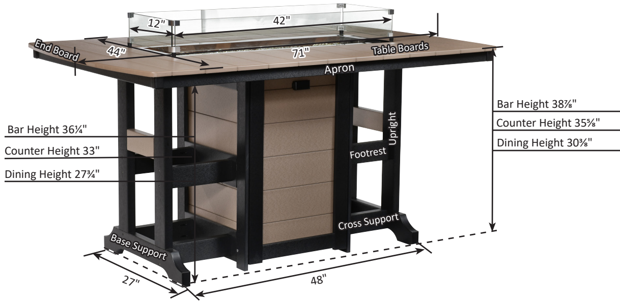
44" x 72" Rectangular Fire Table
