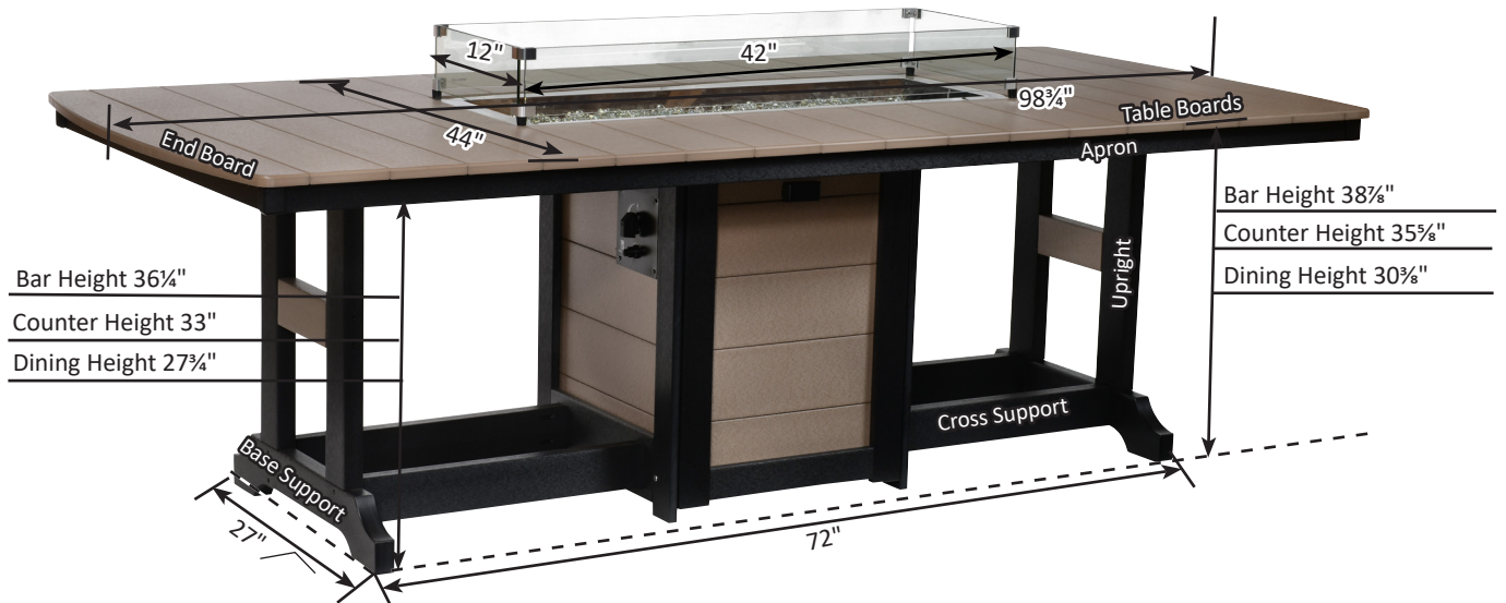
44" x 96" Rectangular Fire Table
