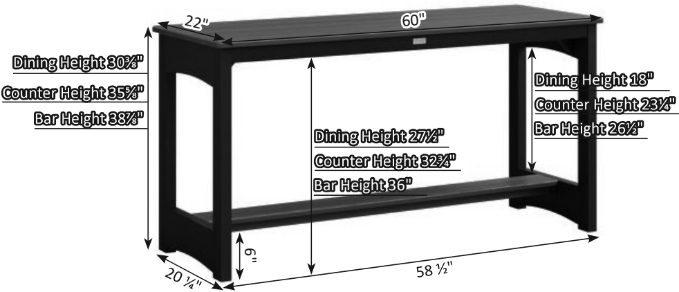
Balcony Table with HDPE Base
