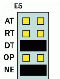
Figure 6 - Header E5, RS-485 'DTR' Enabled, with No Echo
