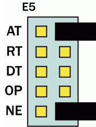
Figure 1 - Header E5, RS-422
