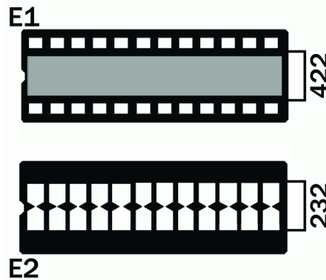
Figure 8 - headers E1 & E2, RS-232 Selected
