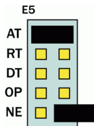
Figure 3 - Header E5, RS-485 'Auto' Enabled, with 'Echo'
