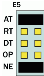
Figure 2 - Header E5, RS-485 'Auto' Enabled, with 'No Echo'
