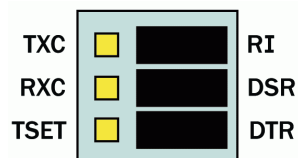
Figure 12 - Header E3, Clocking and Modem control signal selection
