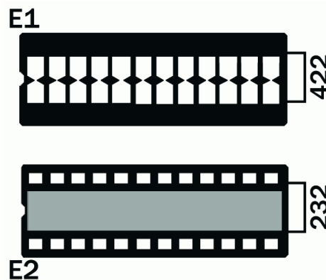
Figure 9 - Headers E1 & E2, RS-422/485 Selected
