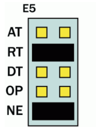
Figure 4 - Header E5, RS-485 'RTS' Enabled, with 'No Echo'
