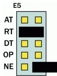
Figure 5 - Header E5, RS-485 'RTS' Enabled, with 'Echo'
