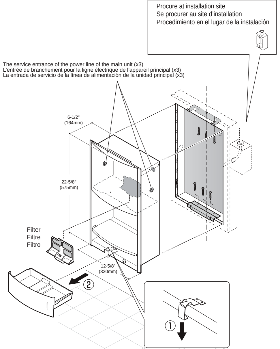
Stringer/additional stud, internal dimension H21-5/8" x W12" (H550 x W305mm) Traverse/Montant supplémentaire dimension intérieure H21-5/8" x W12" (H550 x W305mm) Tirante/Marco adicional dimensión del interior H21-5/8" x W12" (H550 x W305mm)
