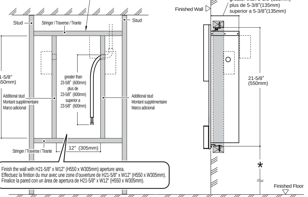
Stringer/additional stud, internal dimension H21-5/8" x W12" (H550 x W305mm) Traverse/Montant supplémentaire dimension intérieure H21-5/8" x W12" (H550 x W305mm) Tirante/Marco adicional dimensión del interior H21-5/8" x W12" (H550 x W305mm)
