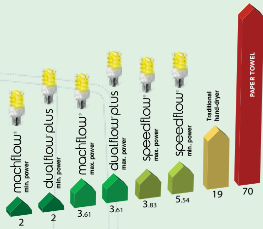
CONSUMPTION IN WATTS PER DRYING CYCLE
