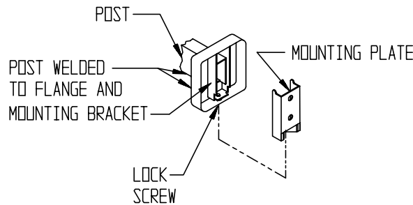
CONCEALED MOUNTING DETAIL
