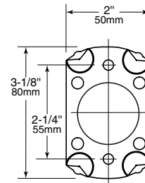
Snap Flange
