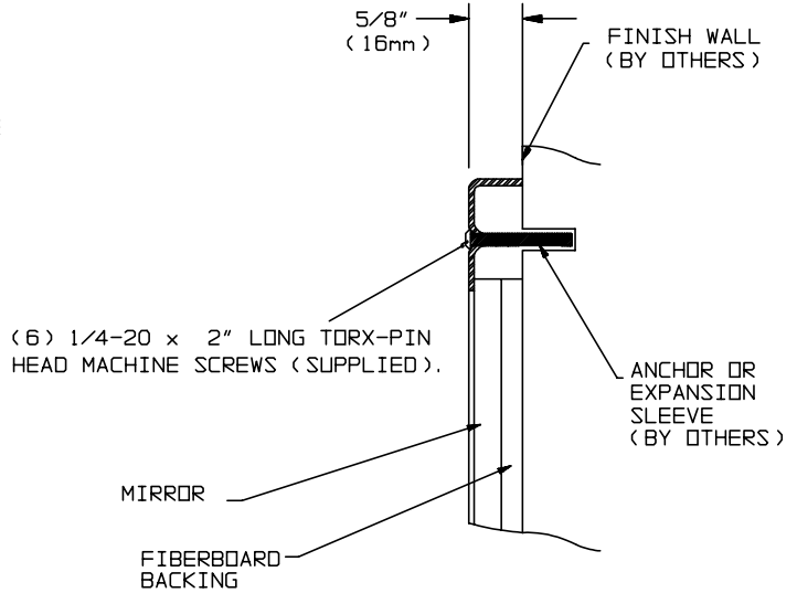
INSTALLATION DETAIL
