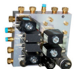
ARGON VALVE BLOCK SMA5 FOR TUBING/ REDUCED CONSTANT FLOW VENTILBLOCK ARGON SMA5/ ROHRMONTAGE / CONSTANT FLOW REDUZIERT
