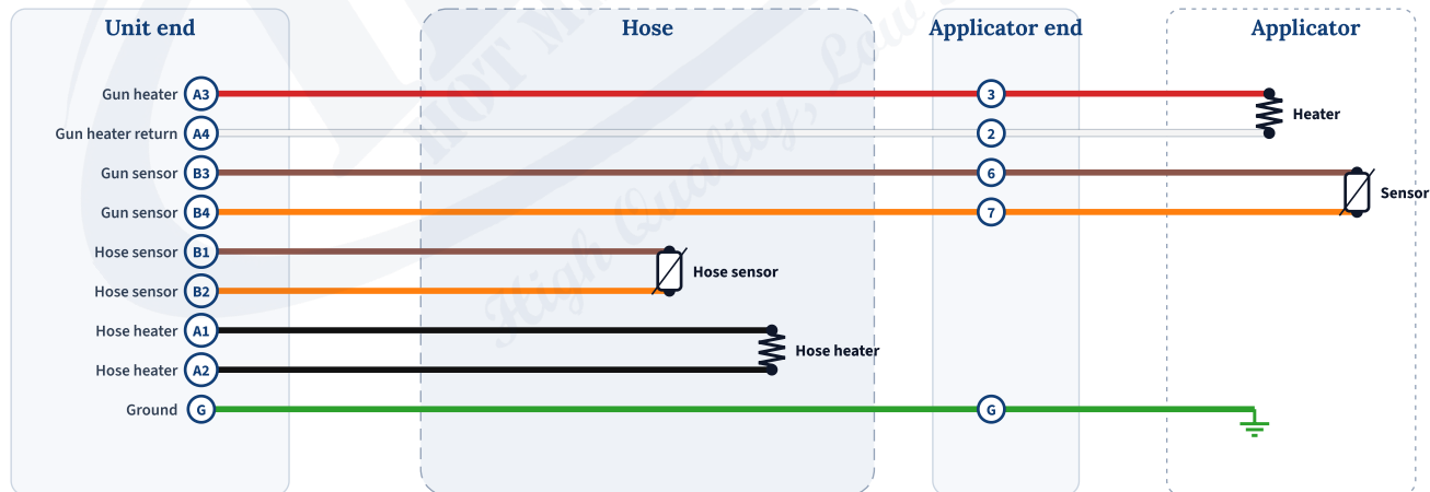
15 pin, unit end (A5, B5, C1 to C5 not used)
