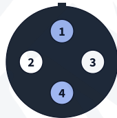
4 pin AMP, pump start
