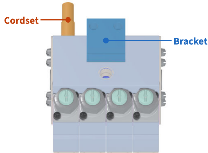
LB: cordset left of the bracket
