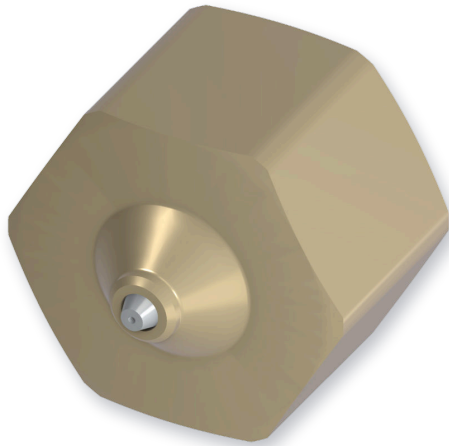
Phosphor brass body, stainless steel insert
