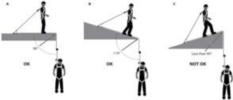
Figure 6 - Leading Edge Angle of Lifeline Redirect
