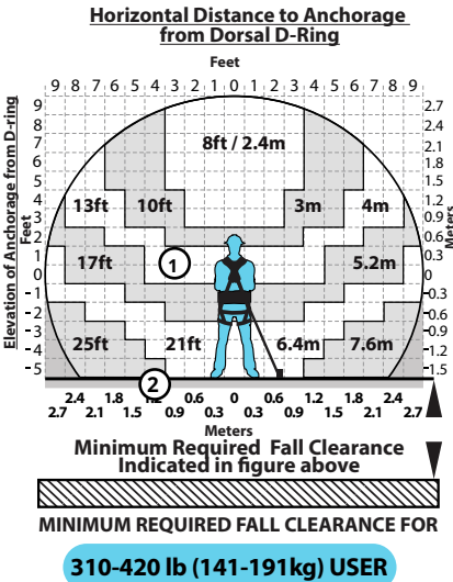
Figure 14 - FT-X Minimum Required Fall Clearance for 310 to 420 lbs. (141 to 191 kg) Users
