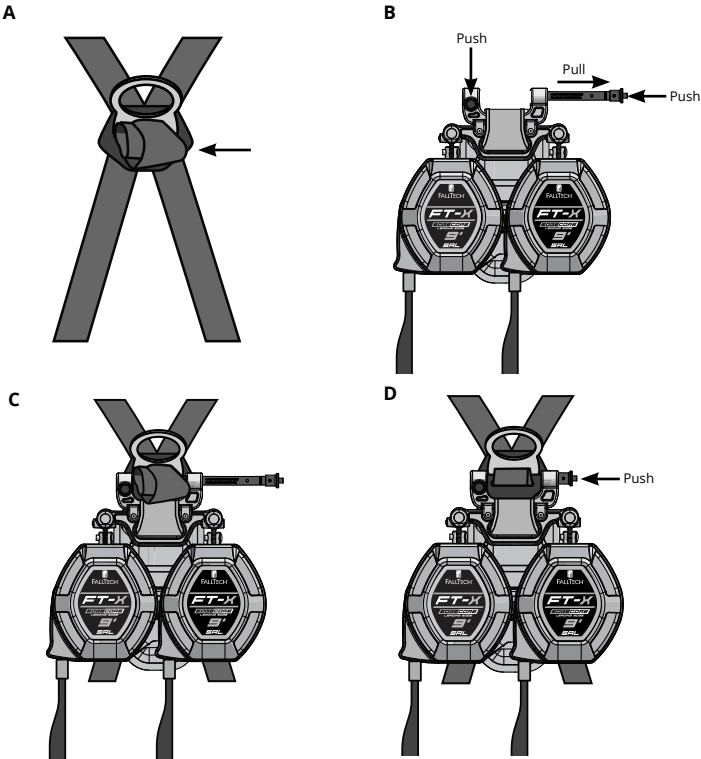
Figure 6 - FT-X EdgeCore Arc Flash Tie-Back Class 2 Leading Edge SRL-P Installation
