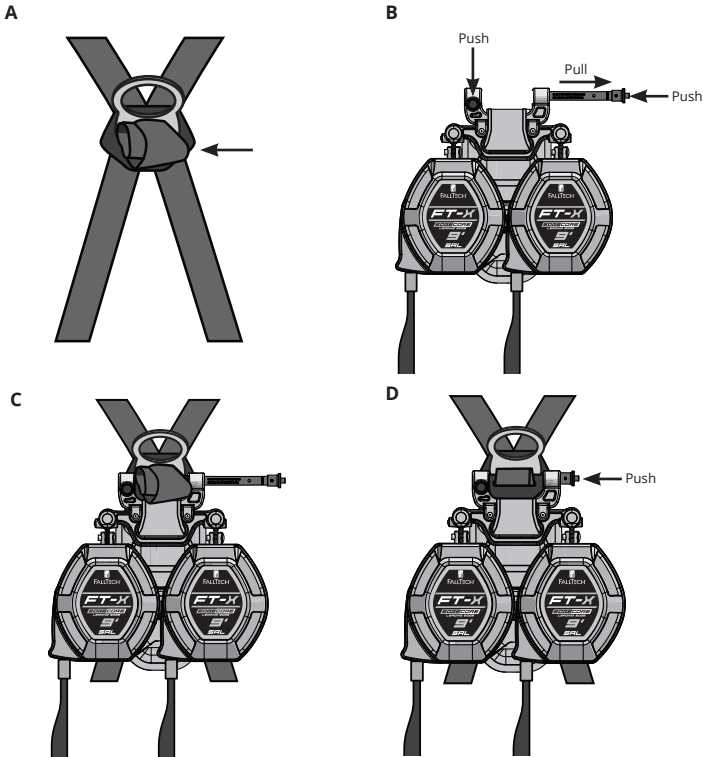
Figure 6 - FT-X™ EdgeCore™ Arc Flash Tie-Back Class 2 Leading Edge SRL-P Installation
