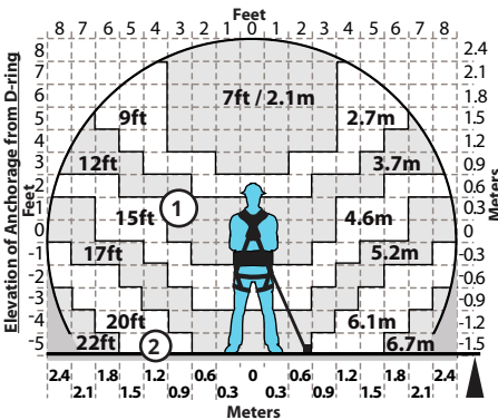
Figure 12 - FT-X Minimum Required Fall Clearance for 130 to 310 lbs. (59 to 141 kg) Users
