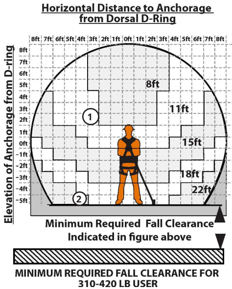
Figure 14 - FT-X Minimum Required Fall Clearance for 310 to 420 lbs. (141 to 191 kg) Users
