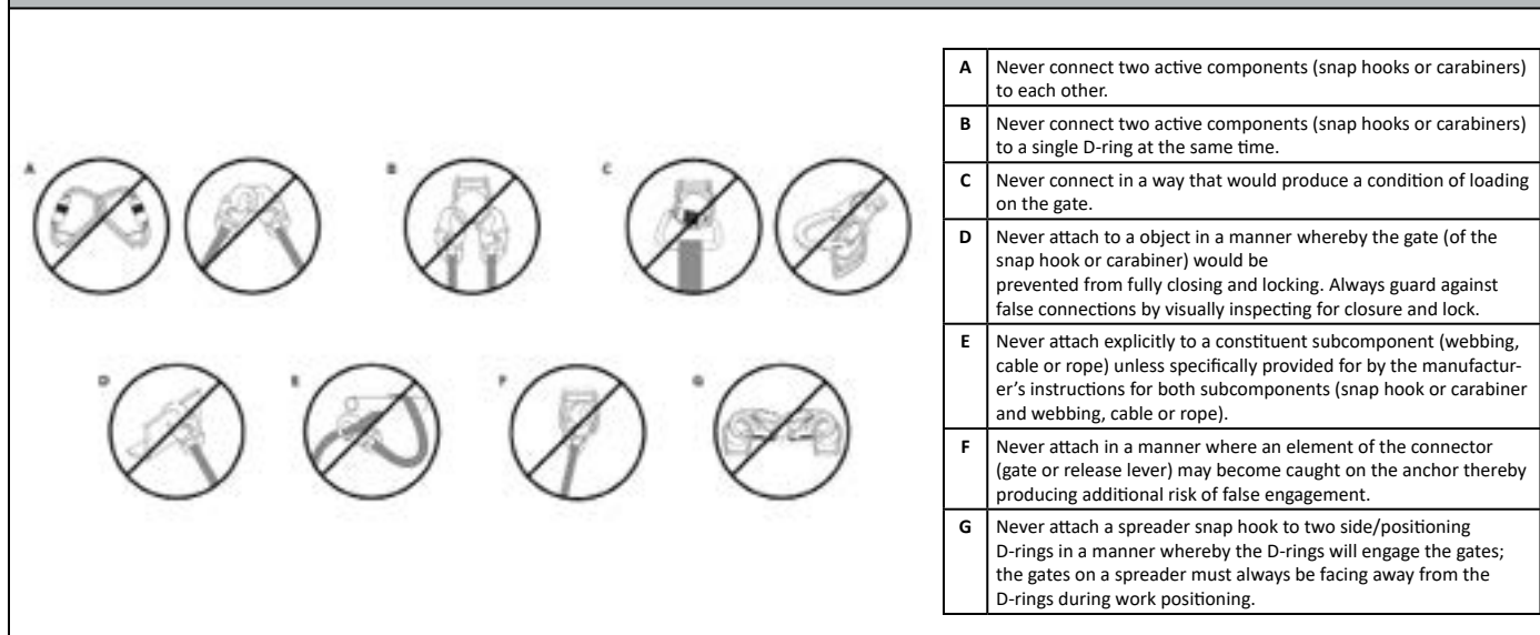
Figure 5 - Non-Compatible Connections
