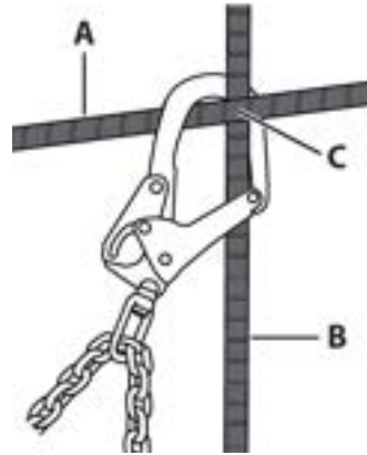
Figure 7 - Best Practice Rebar Hook Attachment
