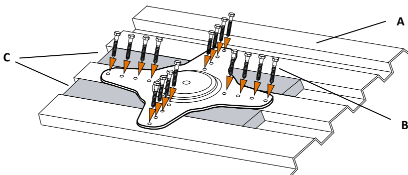
Figure 4 - Steel Decking/Metal Roof Substrate Installation
