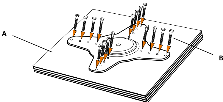
Figure 3 - Wood Roof Substrate Installation
