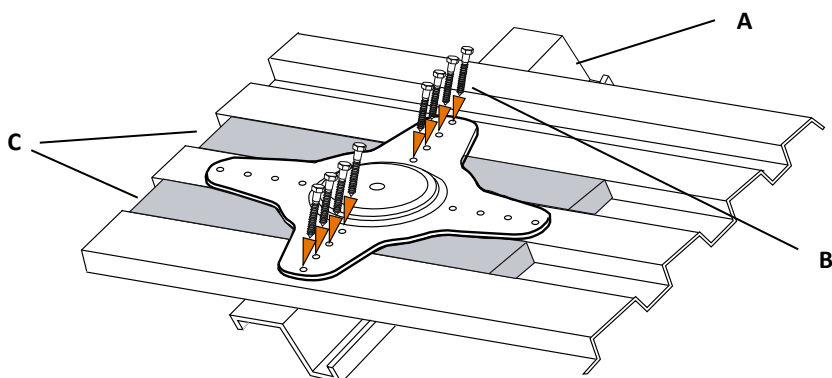
Figure 5 - Steel Z-Purlin Substrate Installation
