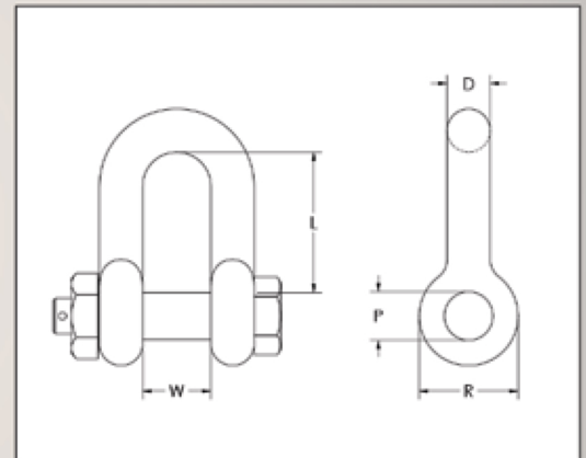
No. 325 Towing Shackle Double Nut with Locking Bolts Available 1 3/4" thru 6 1/2"
