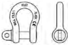
Screwed pin - 122 series
